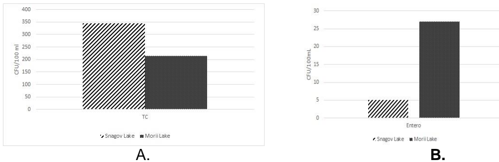
Fig. 4. The densities of A. total coliform bacteria (TC) and B. Enterococci in both natural and anthropogenic lakes during the winter of 2020
